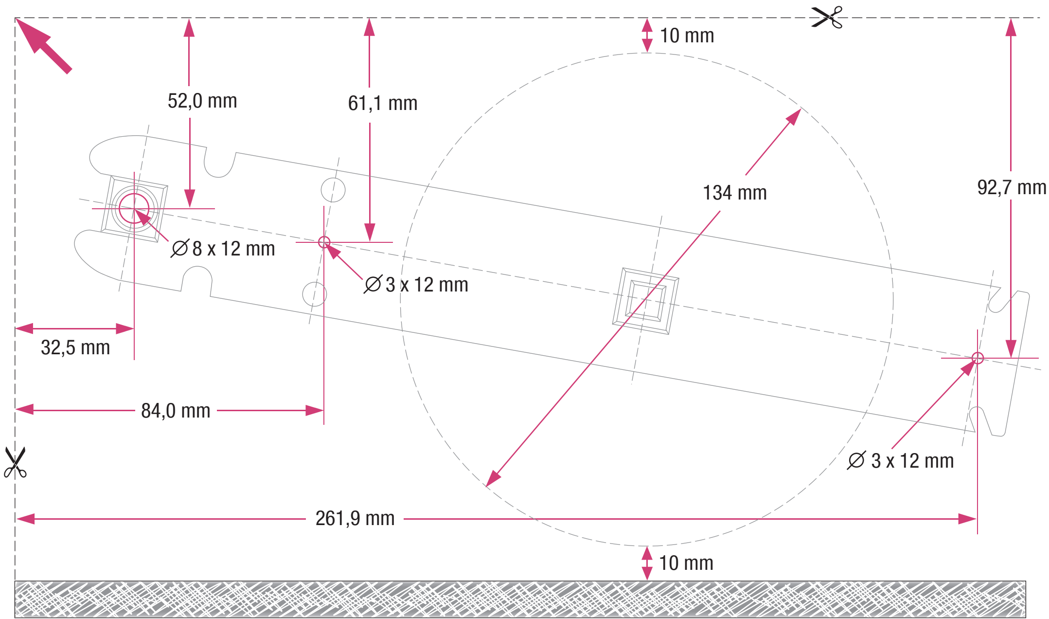
ML 25/1000 Metallic Line 25 mm, SH 1000 mm
